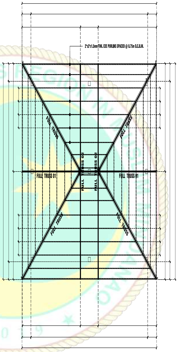
ROOF PLAN SCALE 1:100 MTS.
