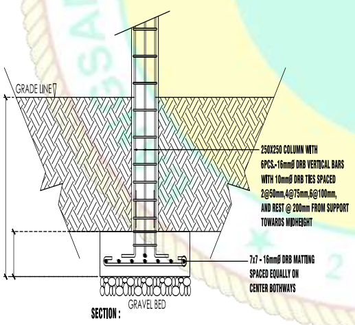
COLUMN-FOOTING DET. SCALE 1:20 MTS.
