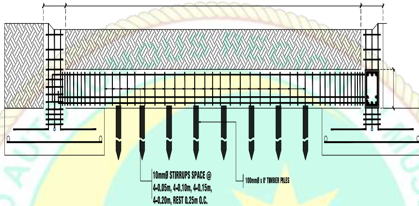
FOOTING TIE BEAM DETAIL SCALE: 1:30 M.
