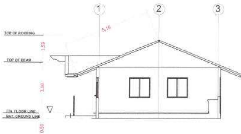
8 CROSS SECTION A-9 SCALE 1:100M
