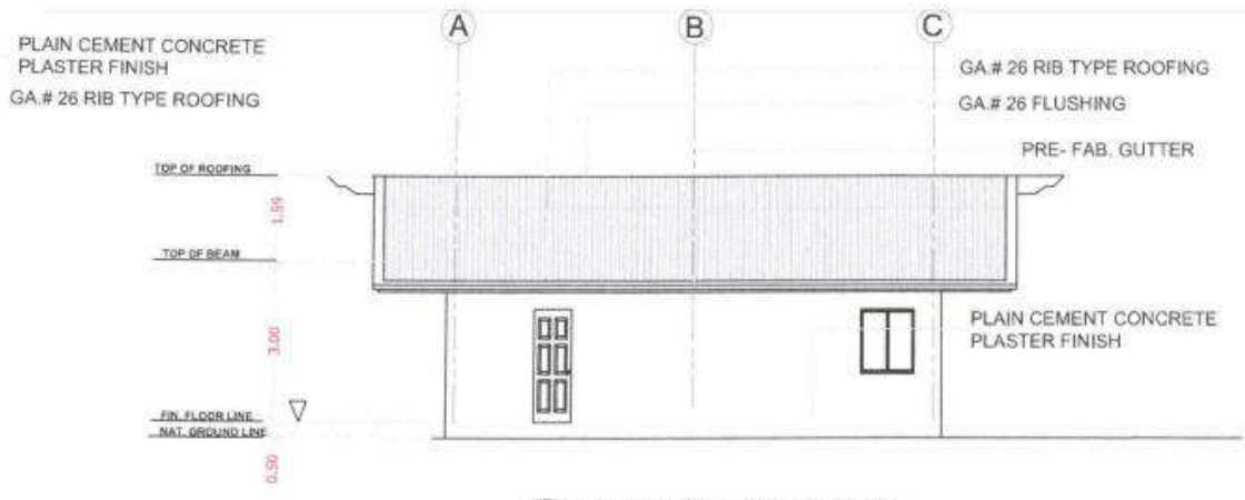
6 REAR SIDE ELEVATION SCALE 1:100 M
