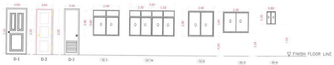
7 S-7 SCALE DOORS AND WINDOW DETAILS 1:100 M
