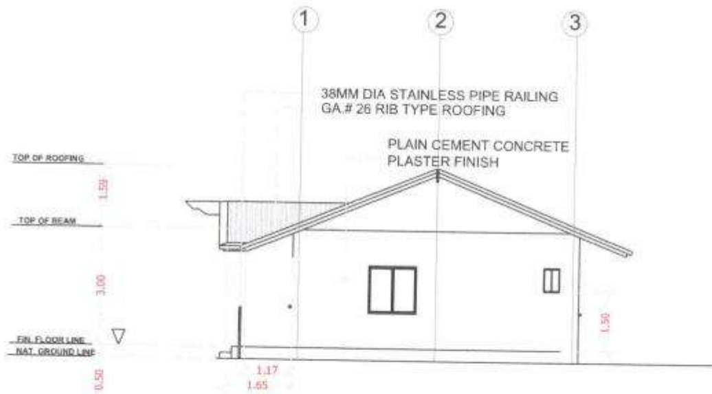
7 RIGHT VIEW ELEVATION A-9 SCALE 1:100M
