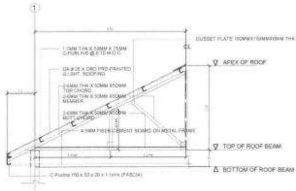
4 S-7 SCALE TYP. TRUSS DETAILS 1:100 M
