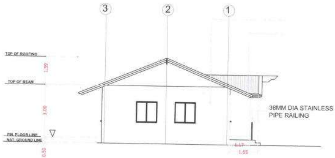
4 LEFT SIDE ELEVATION A-9 SCALE 1:100 M
