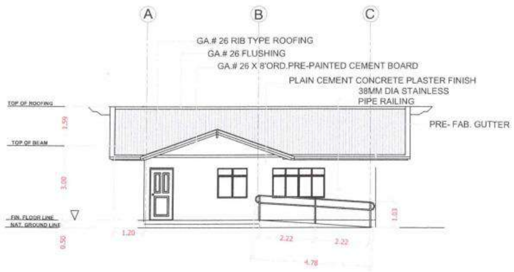
5 FRONT VIEW ELEVATION SCALE 1:100 M
