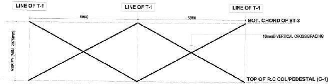
B TYP. DET. OF VERT. CROSS BRACING
