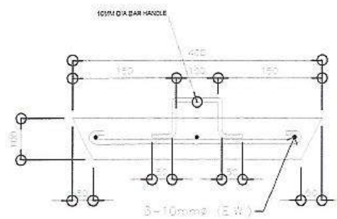
3 DETAILS OF MANHOLE P-3 SCALE 1 : 100 M
