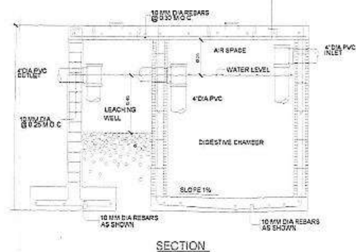
2 DETAILS OF SEPTIC TANK P-3 SCALE 1:100M
