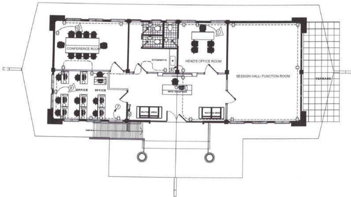
2 POWER LAYOUT PLAN E-3 SCALE 1:100 M
