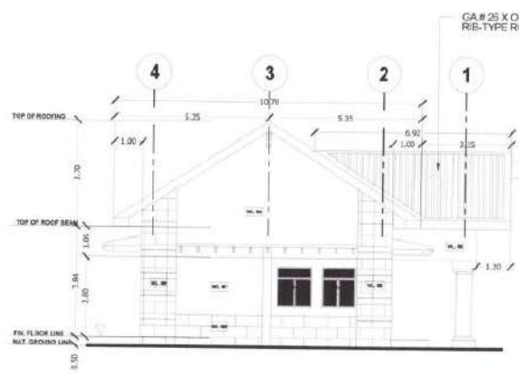
5 LEFT SIDE ELEVATION SCALE 1:100 M
