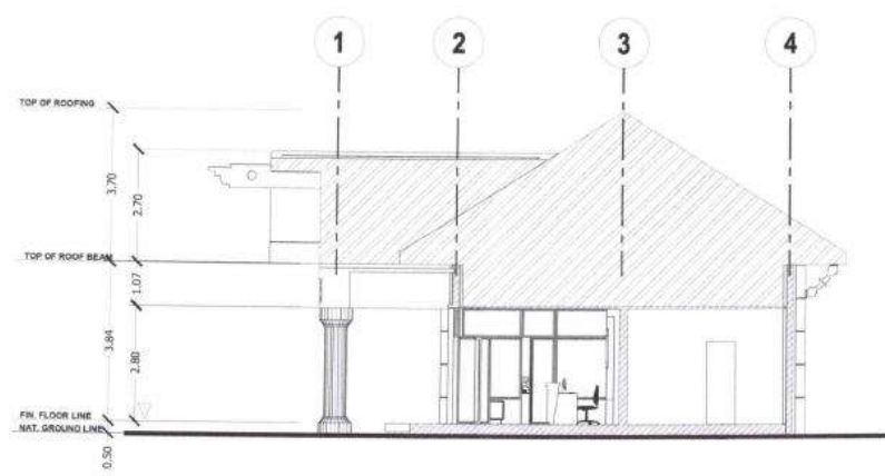
7 CROSS SECTION A-8 SCALE 1:100 M
