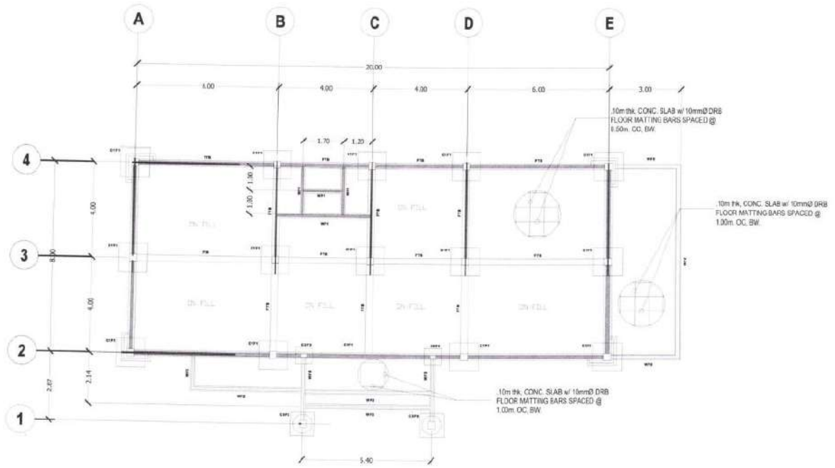
3 FOUNDATION PLAN S-8 SCALE 1:100W
