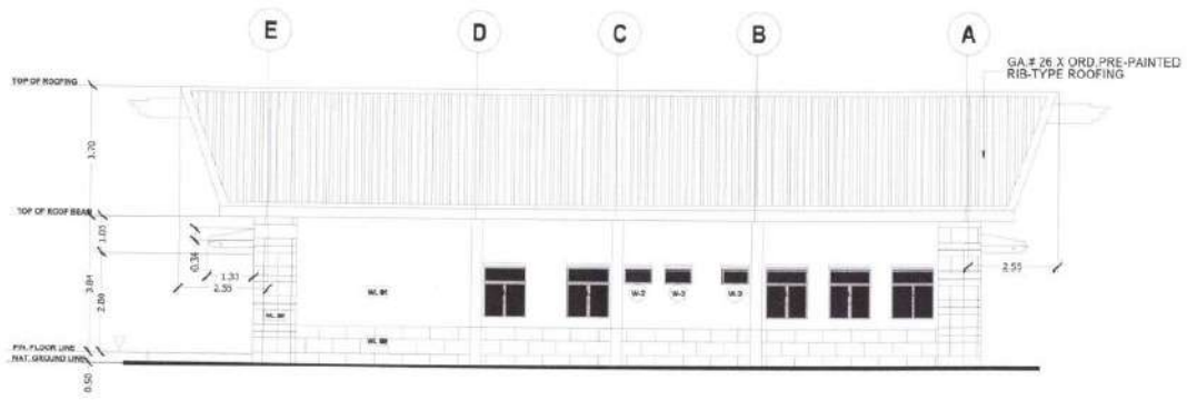
4 REAR ELEVATION A-8 SCALE 1:100 R
