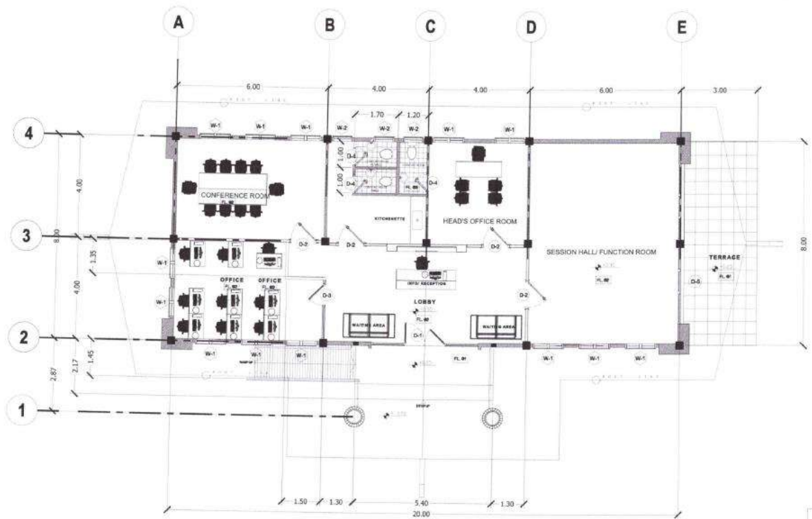
2 GROUND FLOOR PLAN SCALE 1:100 M
