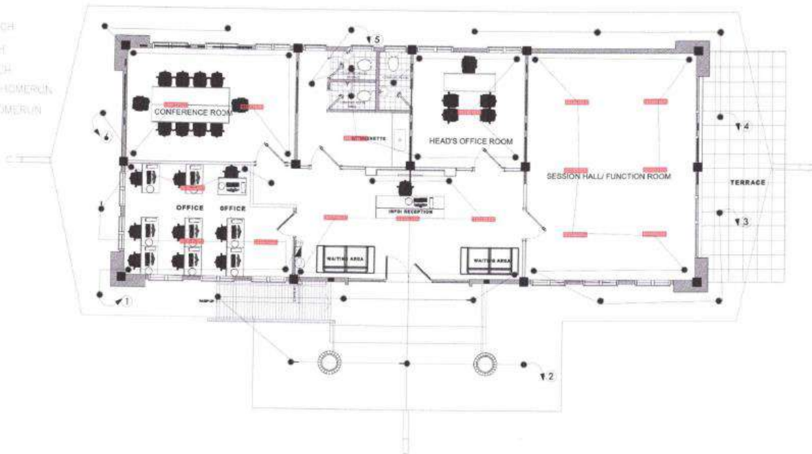
1 LIGHTING LAYOUT PLAN E-3 SCALE 1:100 M
