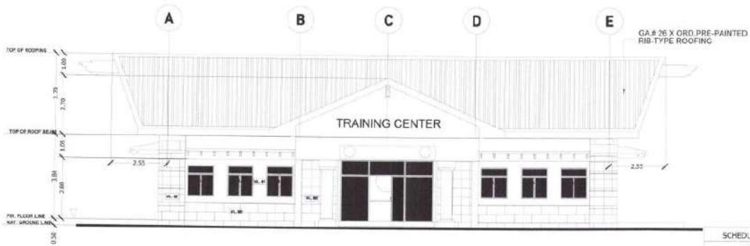
3 FRONT ELEVATION A-8 SCALE 1:100 R
