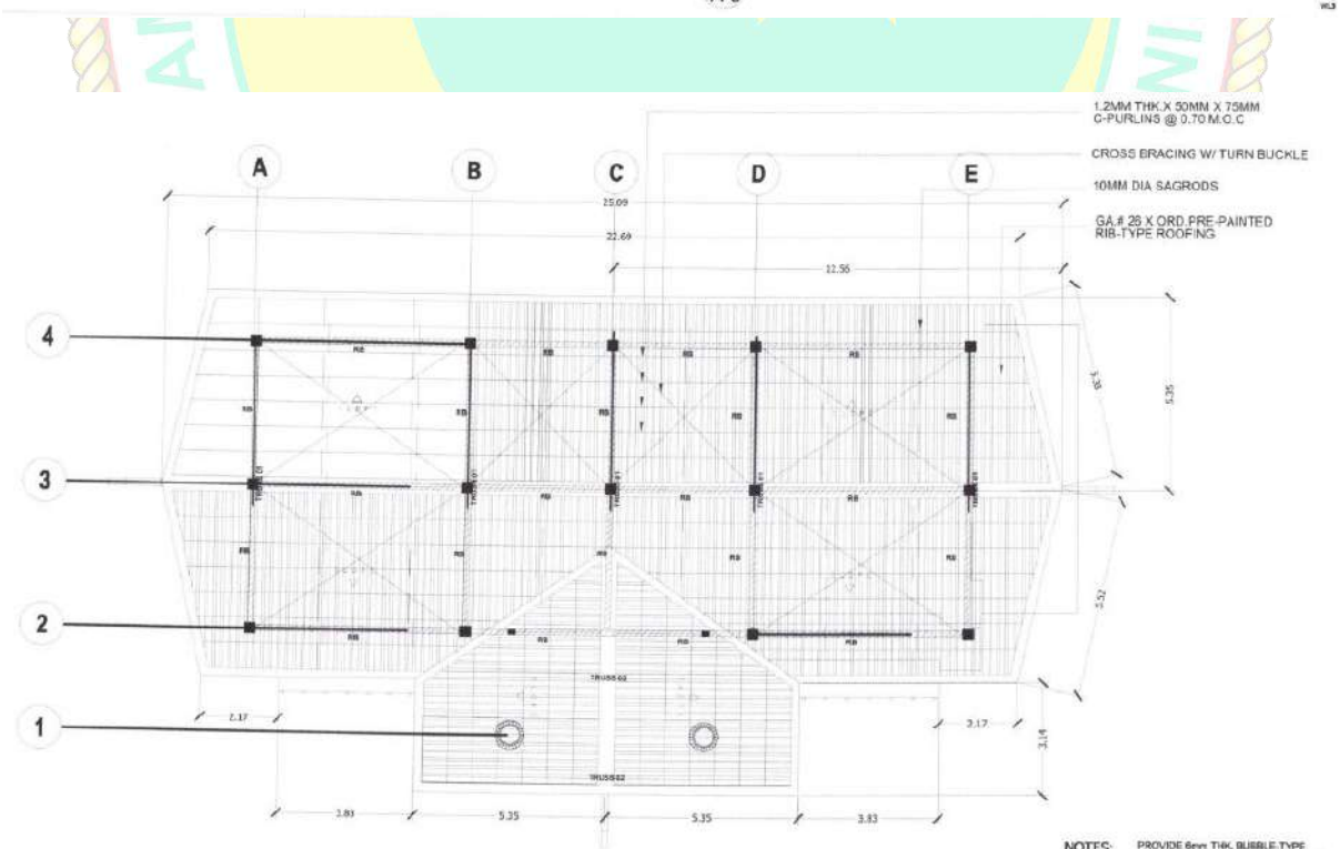
1 ROOF FRAMING LAYOUT PLAN S-8 SCALE 1:100 M
