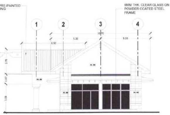
6 RIGHT SIDE ELEVATION SCALE 1:100 M
