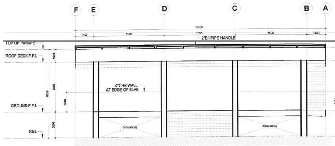
2 REAR ELEVATION SCALE: NTS
