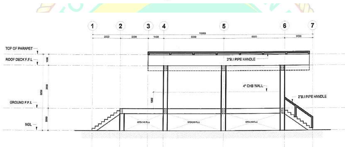
3 TYP. SIDE ELEVATION SCALE: NTS
