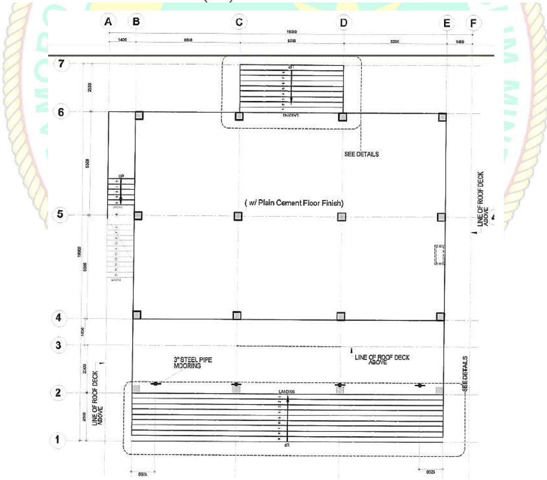
1 GROUND FLOOR PLAN SCALE: 1:100
