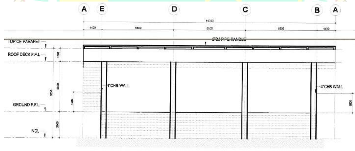
1 FRONT ELEVATION SCALE: R/S
